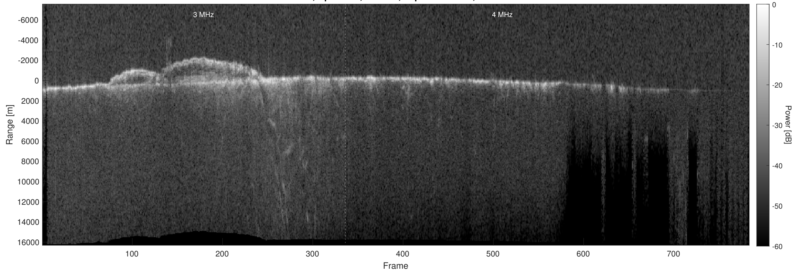
Orbit 9585, Optimized, Window, Depth-Corrected, Channel 2
