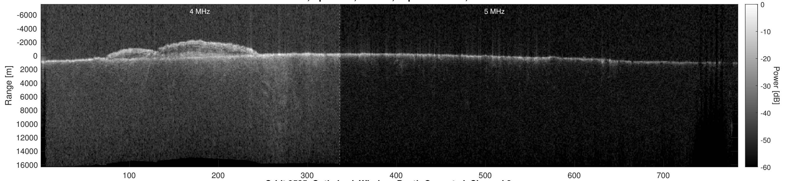
Orbit 9585, Optimized, Window, Depth-Corrected, Channel 2
