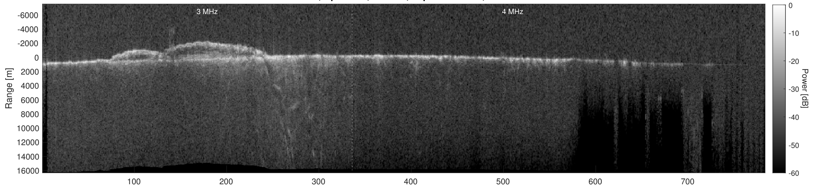
Orbit 9585, Depth-Corrected Cluttergram
