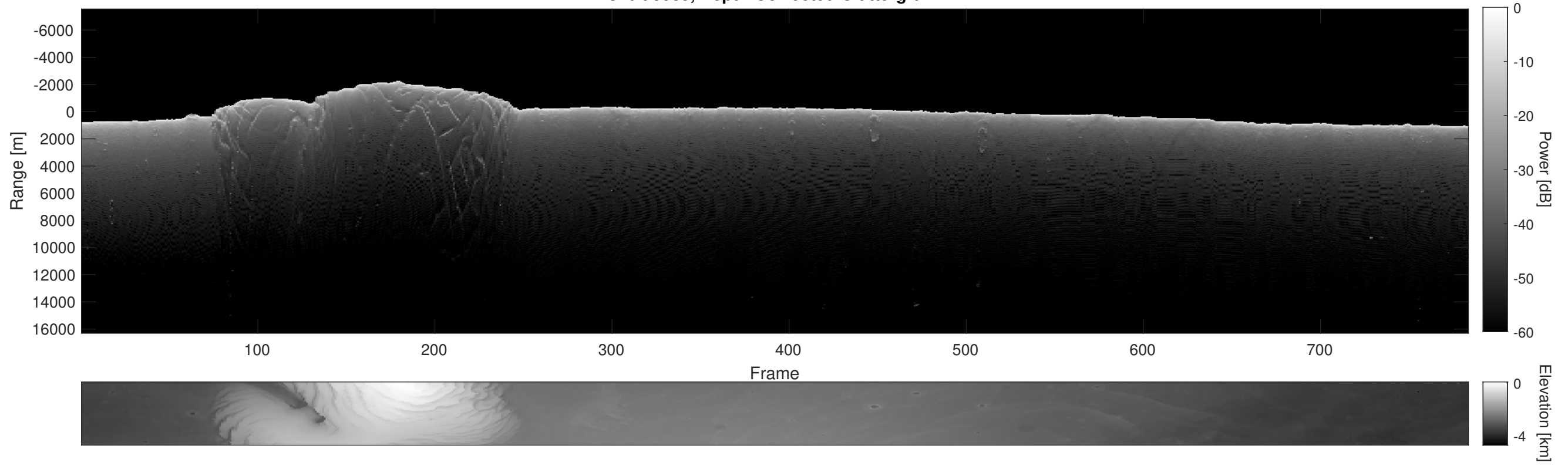
Orbit 9585, Depth-Corrected Cluttergram
