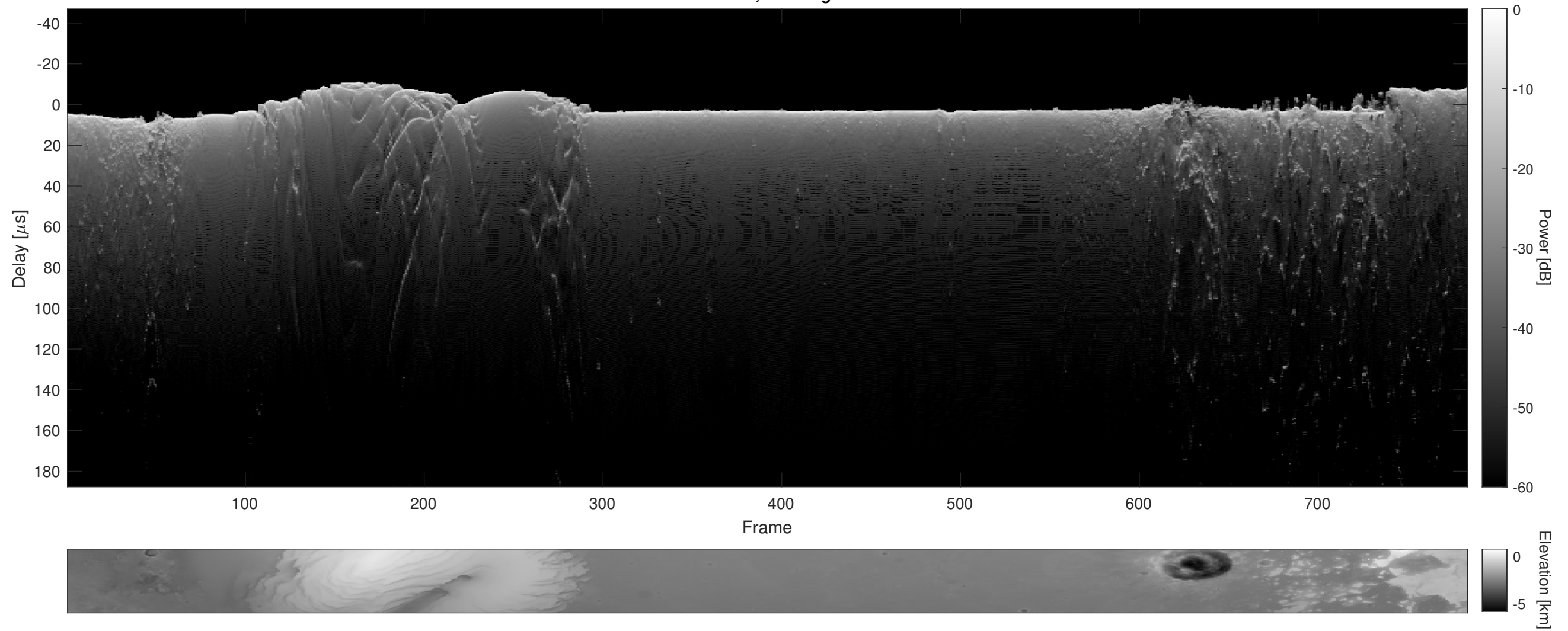
Orbit 9586, Cluttergram
