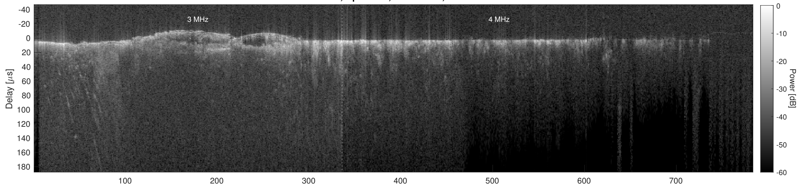
Orbit 9586, Cluttergram
