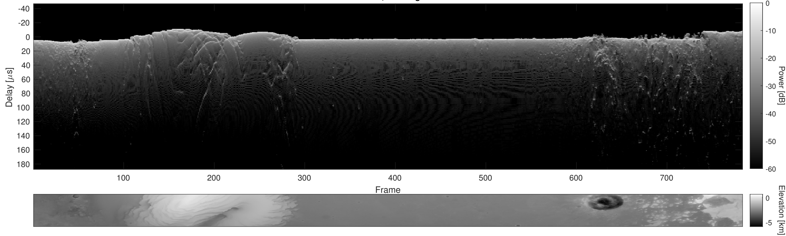
Orbit 9586, Cluttergram
