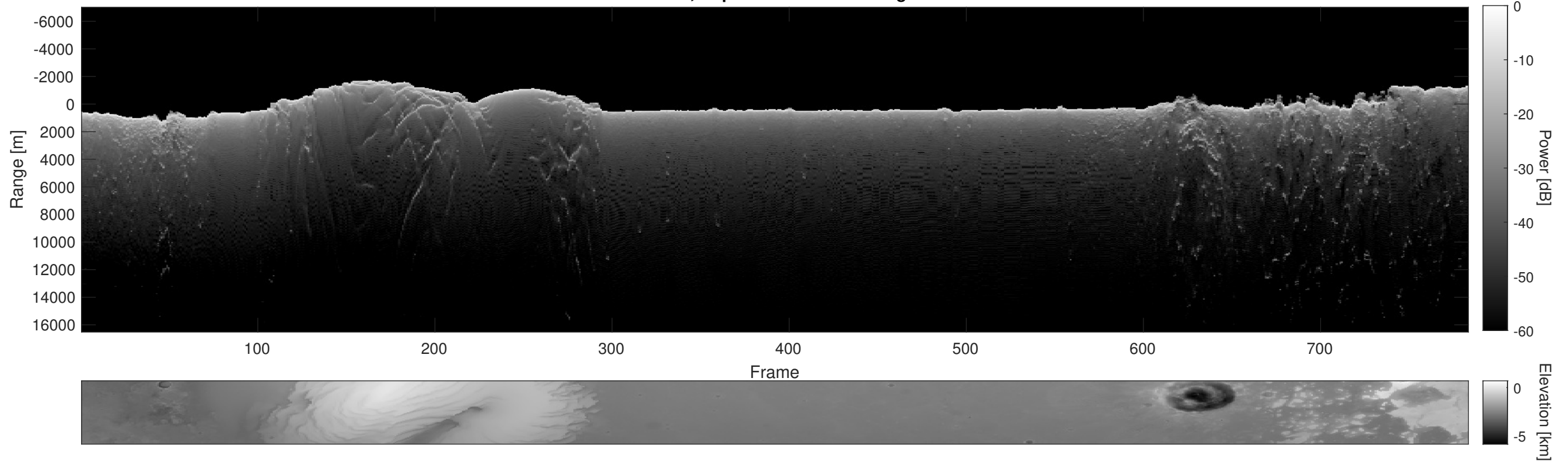
Orbit 9586, Depth-Corrected Cluttergram
