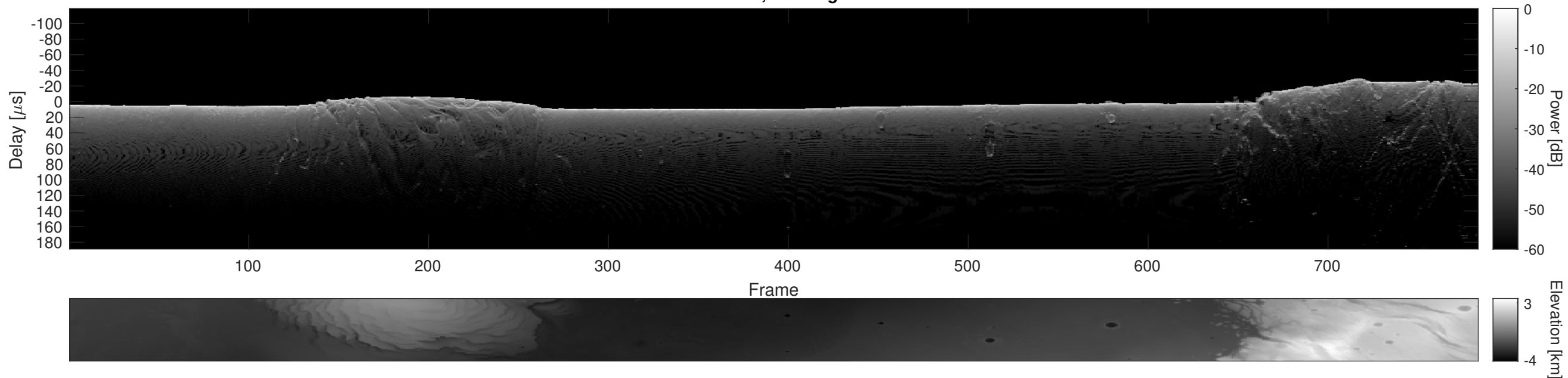
Orbit 9587, Cluttergram
