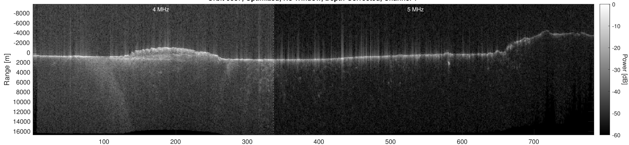
Orbit 9587, Optimized, No Window, Depth-Corrected, Channel 2
