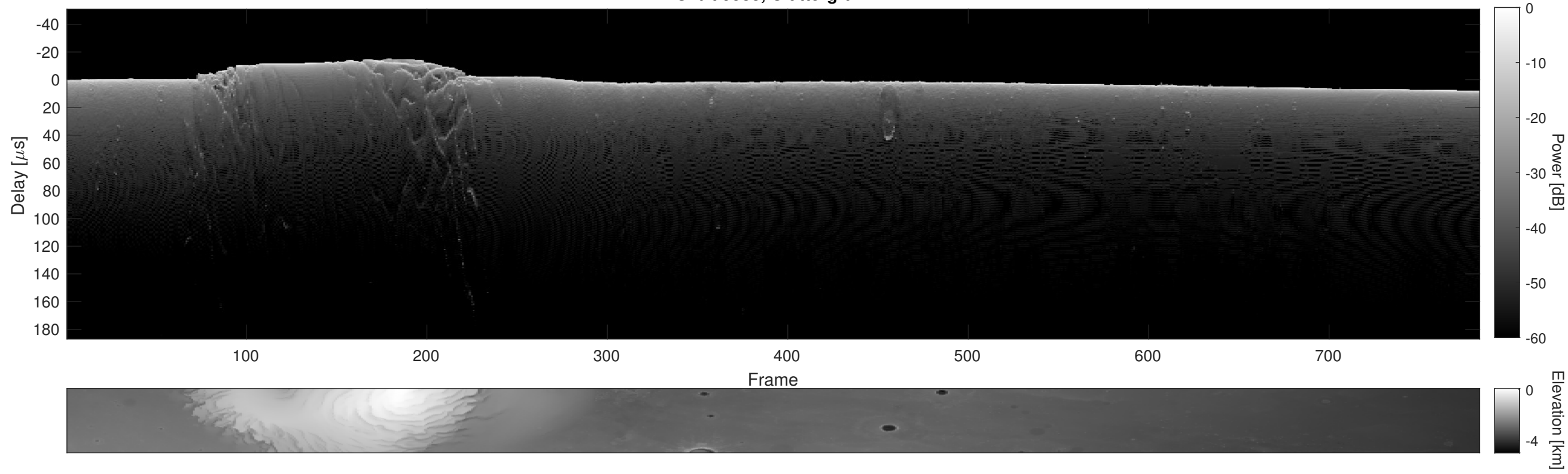
Orbit 9588, Cluttergram
