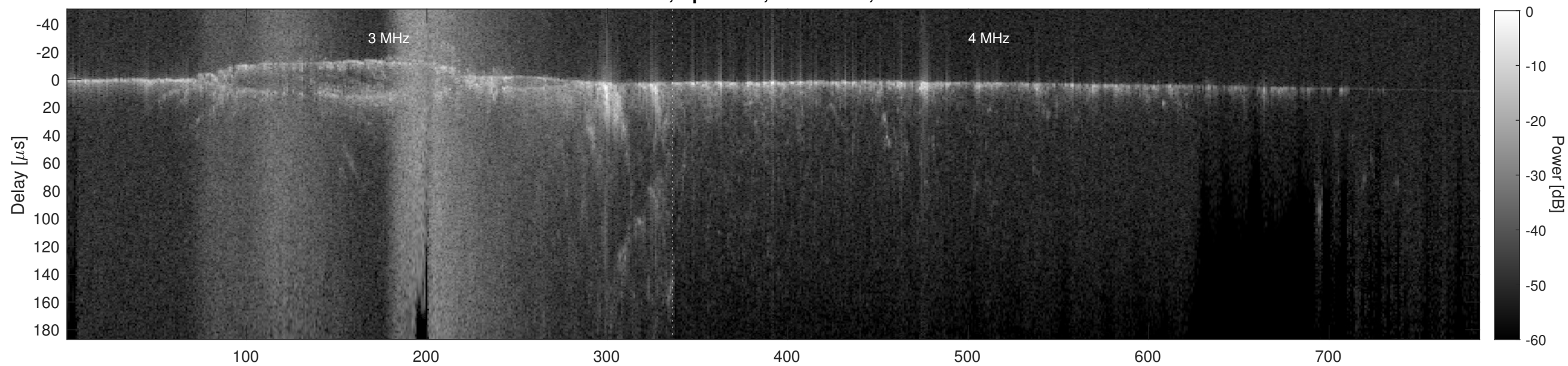
Orbit 9588, Cluttergram
