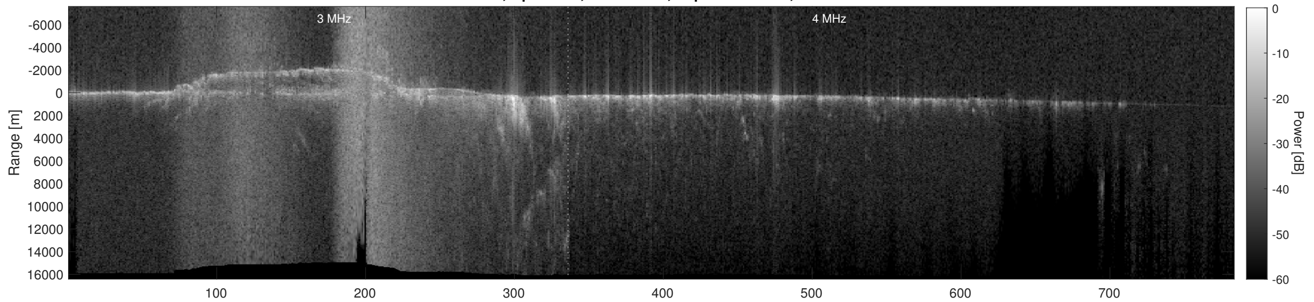
Orbit 9588, Depth-Corrected Cluttergram
