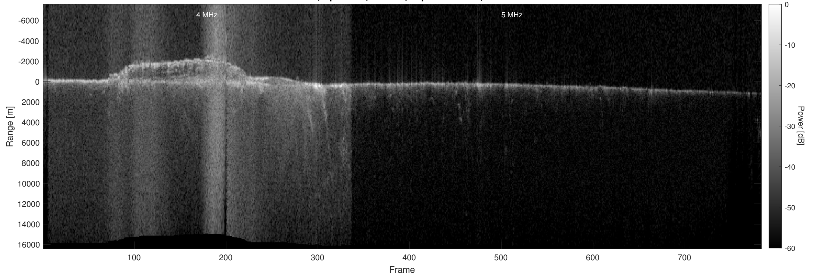
Orbit 9588, Optimized, Window, Depth-Corrected, Channel 2
