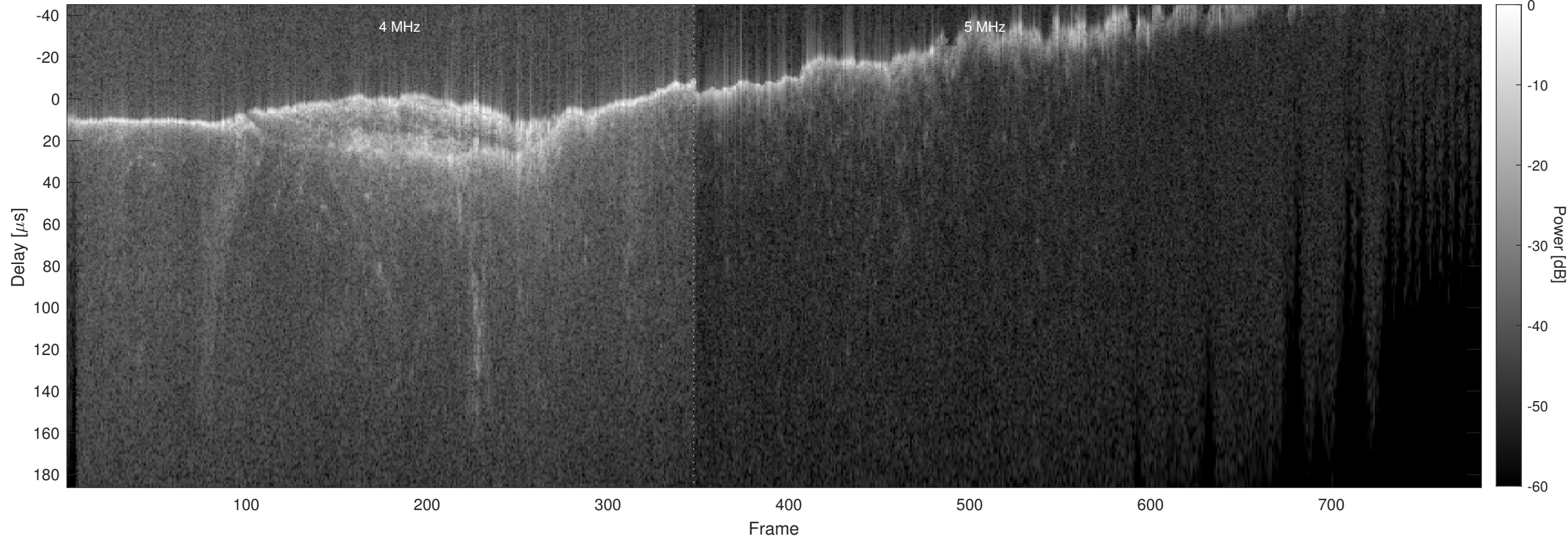
Orbit 9589, Chapman, No Window, Channel 2
