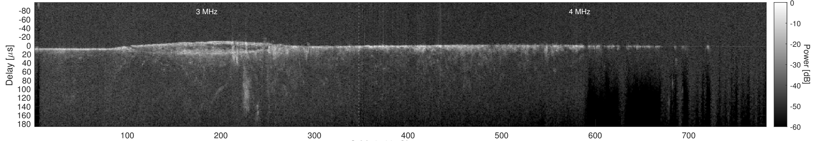
Orbit 9589, Cluttergram
