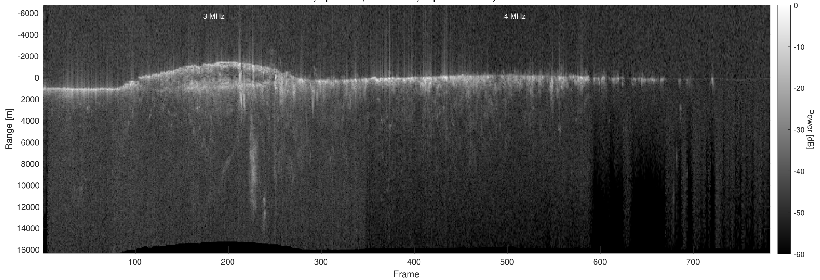
Orbit 9589, Optimized, No Window, Depth-Corrected, Channel 2
