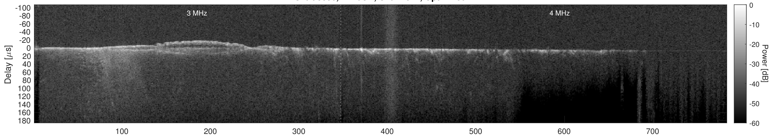
Orbit 9590, Cluttergram
