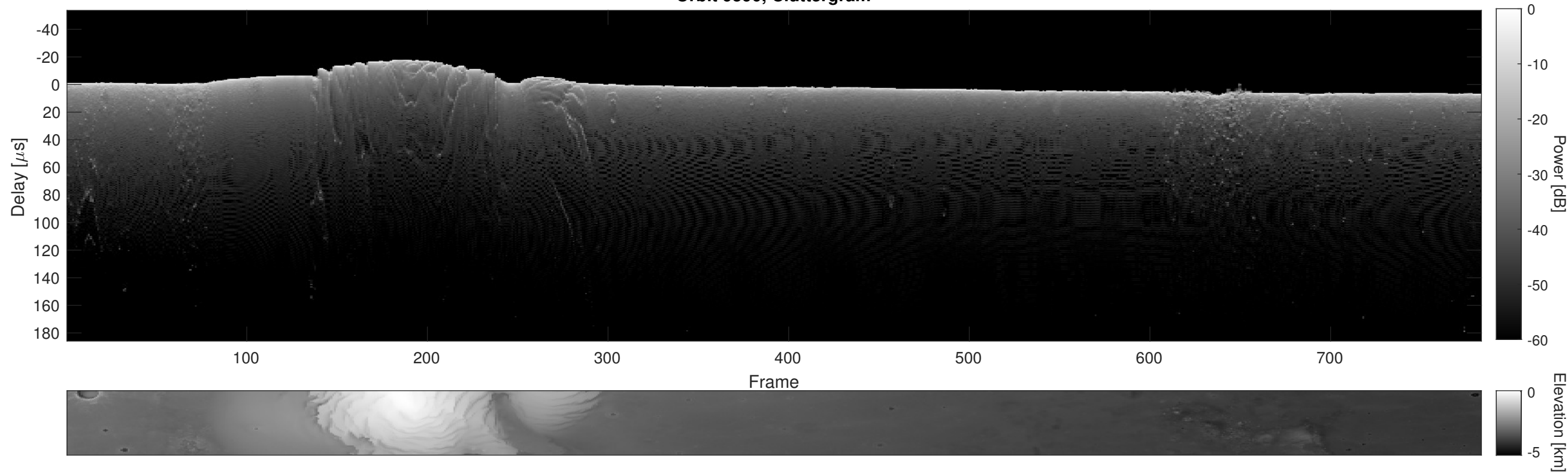
Orbit 9590, Cluttergram
