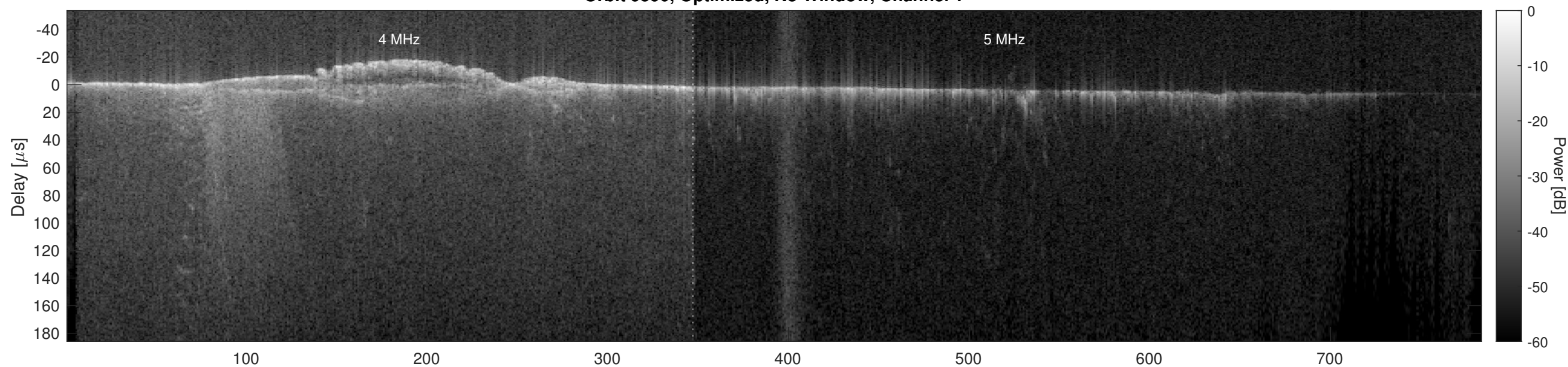
Orbit 9590, Optimized, No Window, Channel 2
