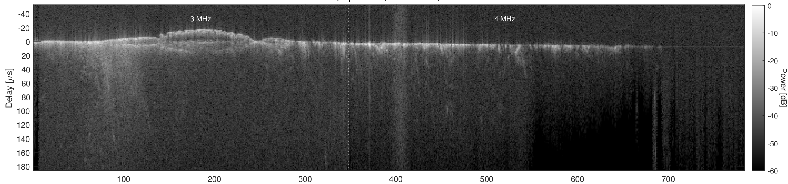
Orbit 9590, Cluttergram
