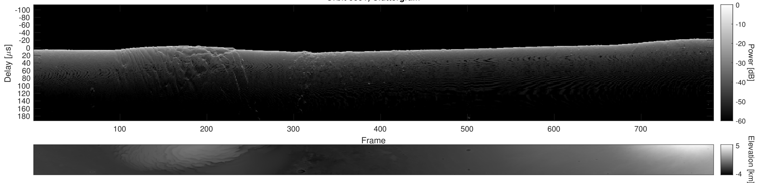
Orbit 9591, Cluttergram
