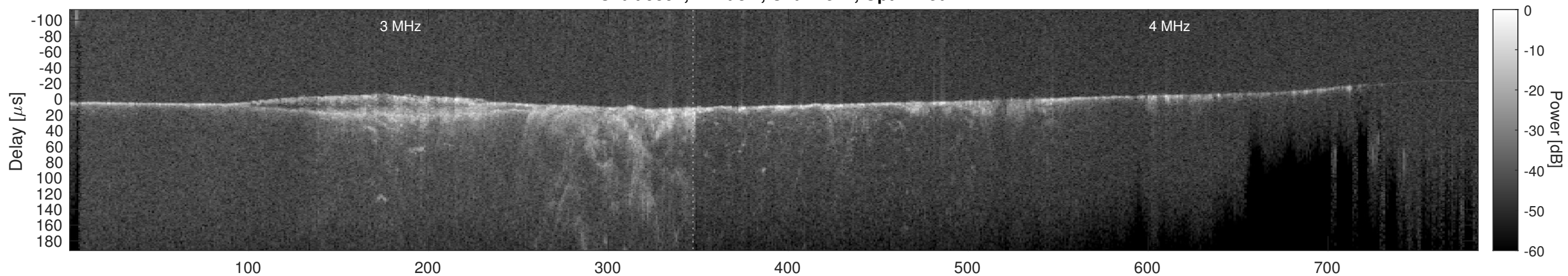
Orbit 9591, Cluttergram
