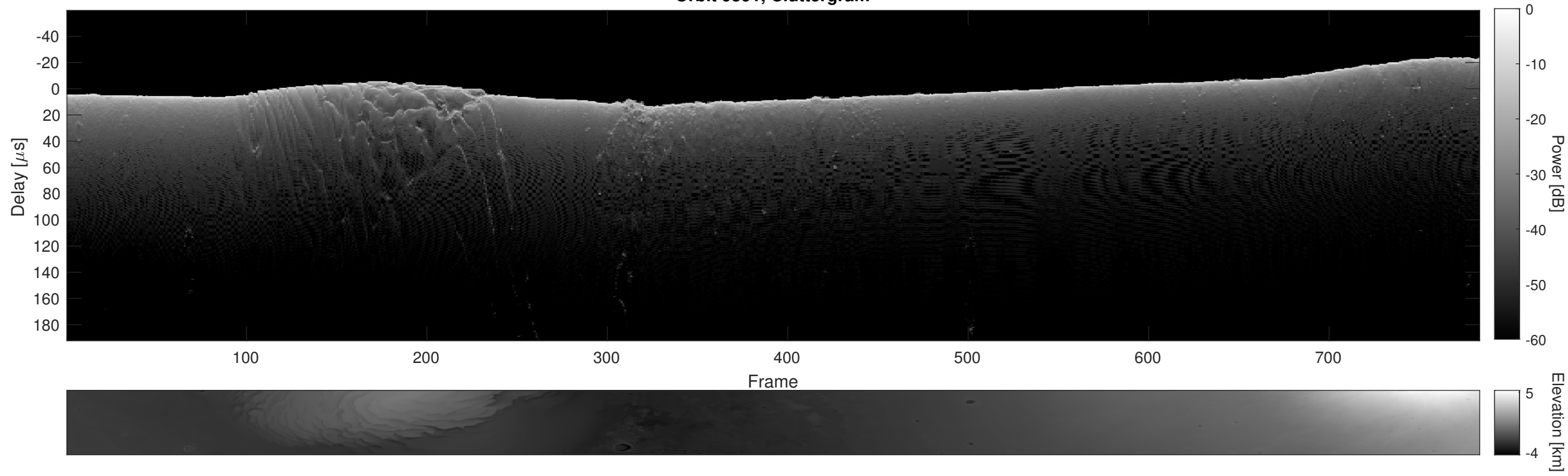
Orbit 9591, Cluttergram
