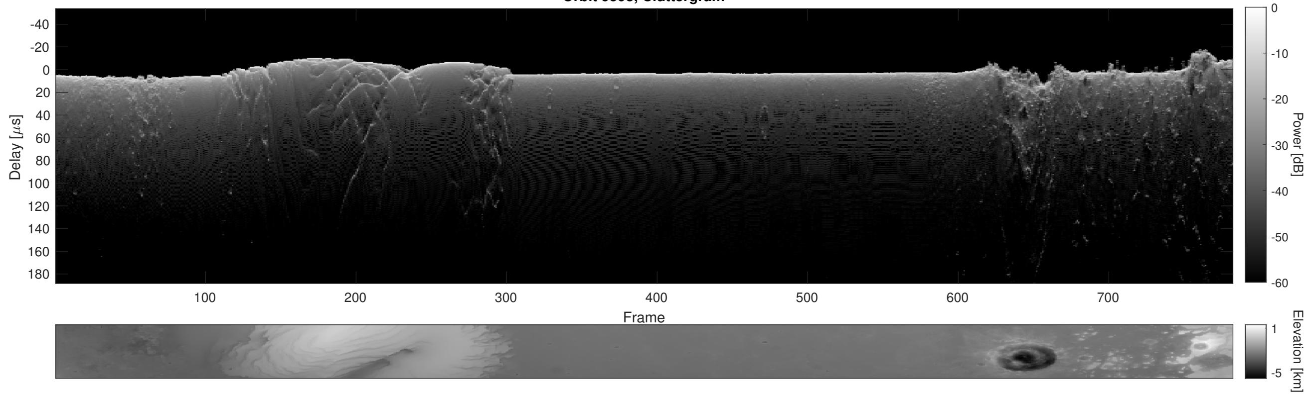
Orbit 9593, Cluttergram
