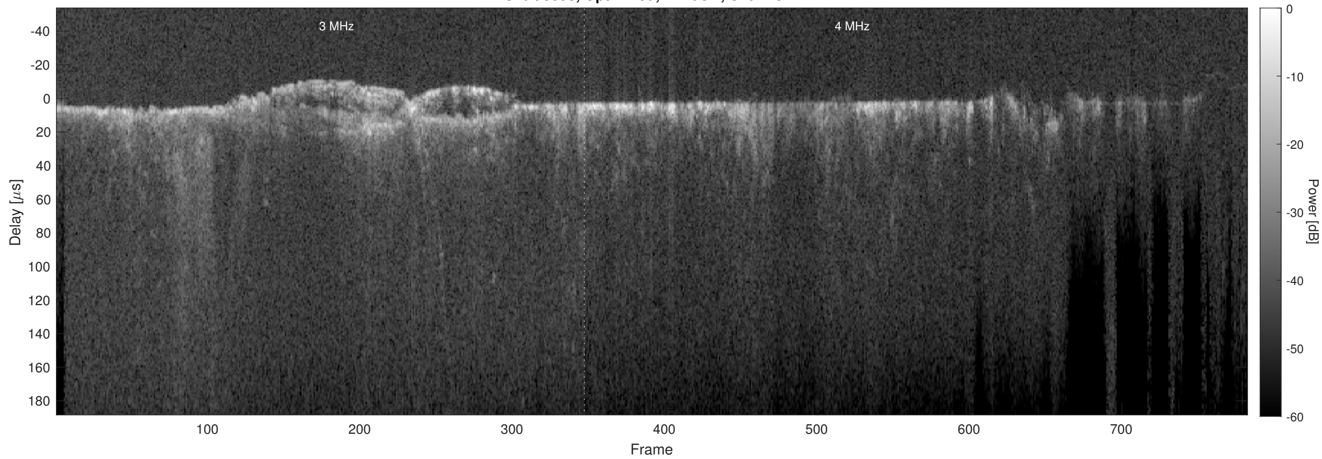
Orbit 9593, Optimized, Window, Channel 2
