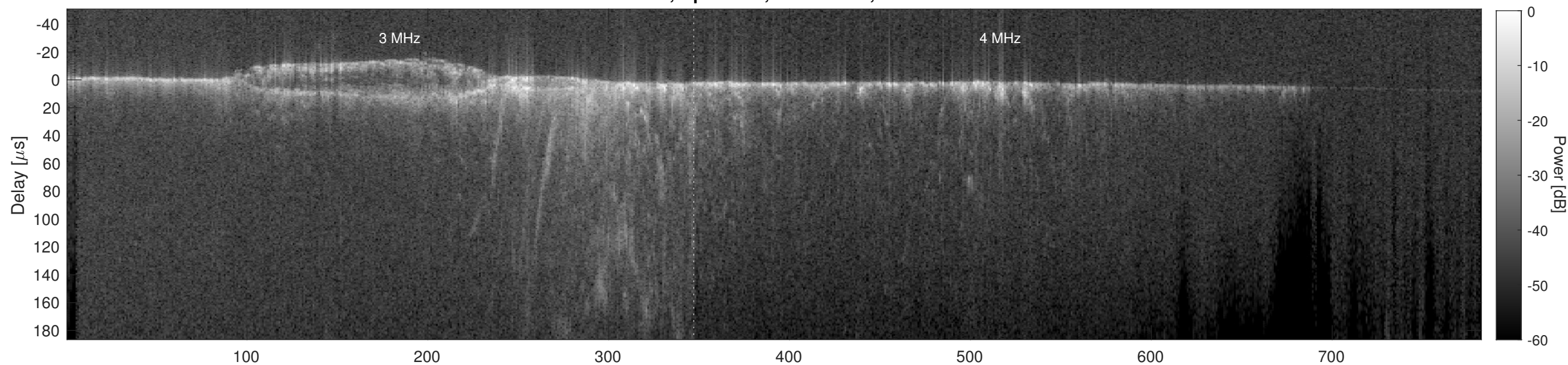
Orbit 9595, Cluttergram
