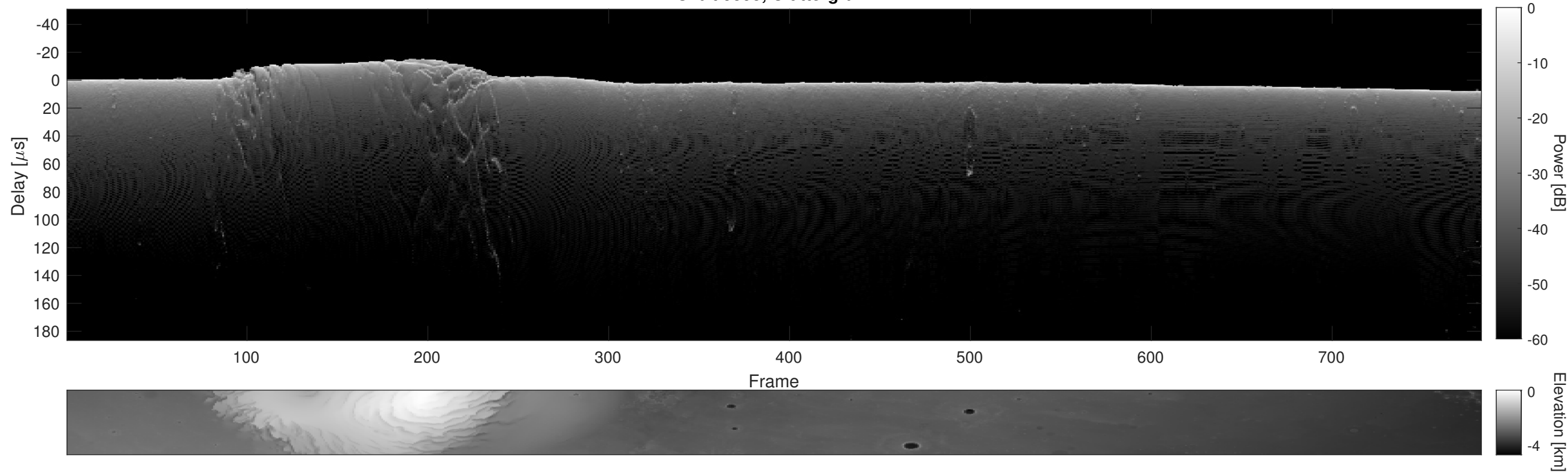
Orbit 9595, Cluttergram
