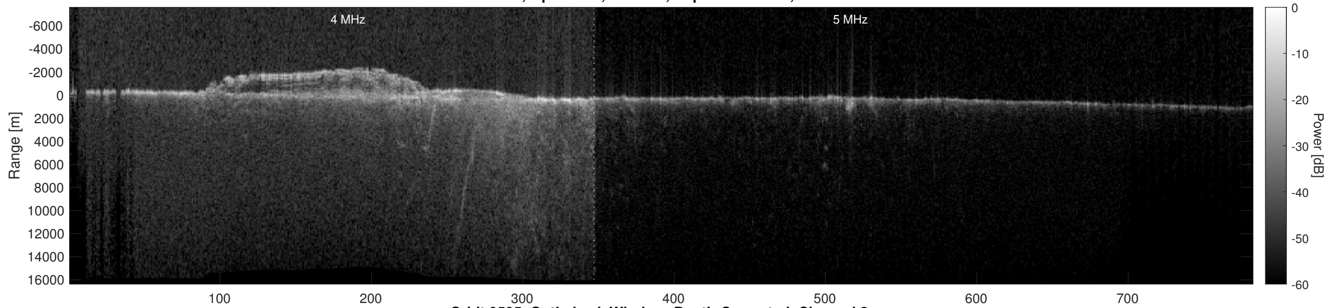
Orbit 9595, Optimized, Window, Depth-Corrected, Channel 2
