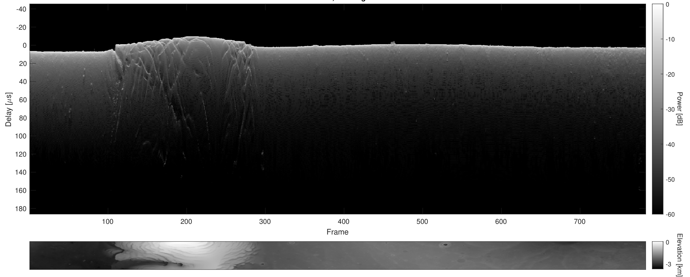
Orbit 9596, Cluttergram
