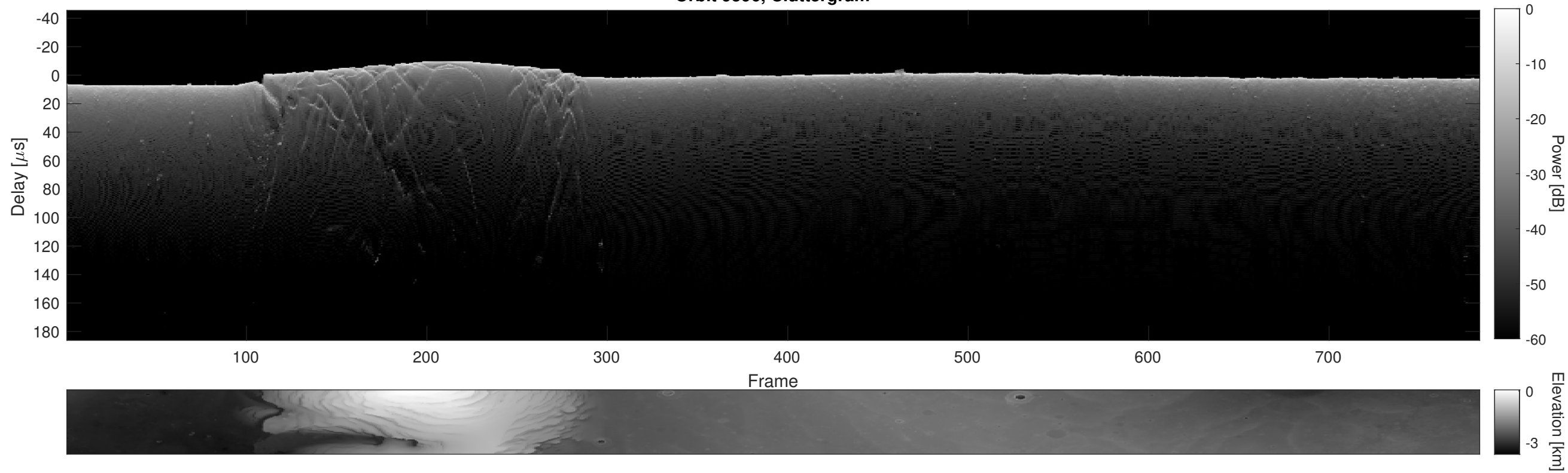
Orbit 9596, Cluttergram
