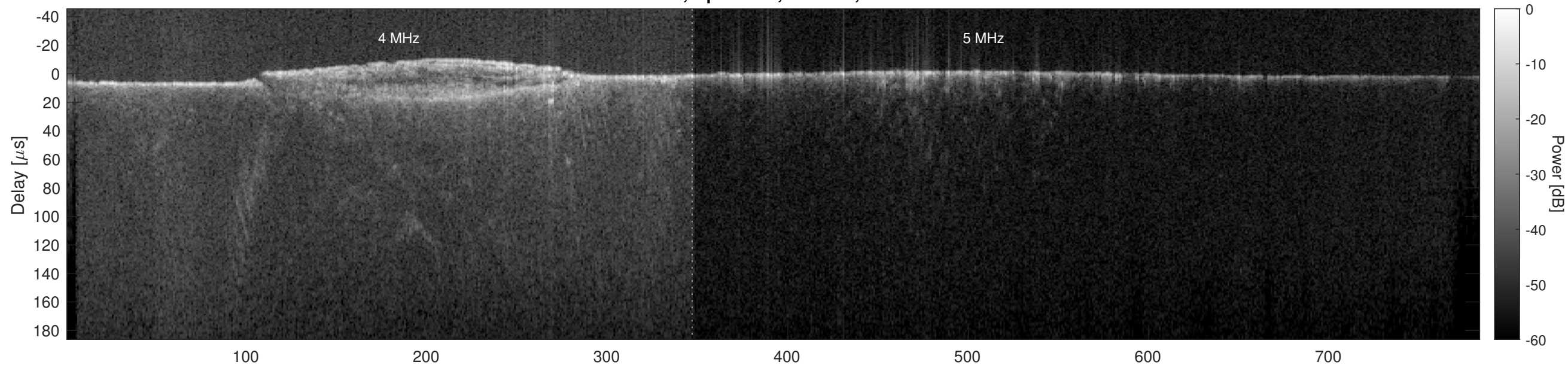
Orbit 9596, Optimized, Window, Channel 2
