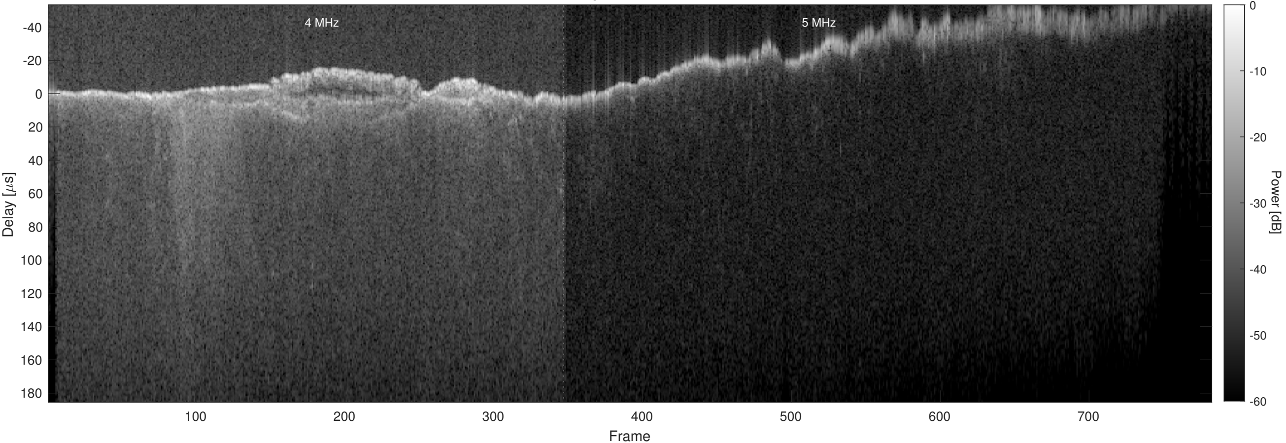
Orbit 9597, Chapman, Window, Channel 2
