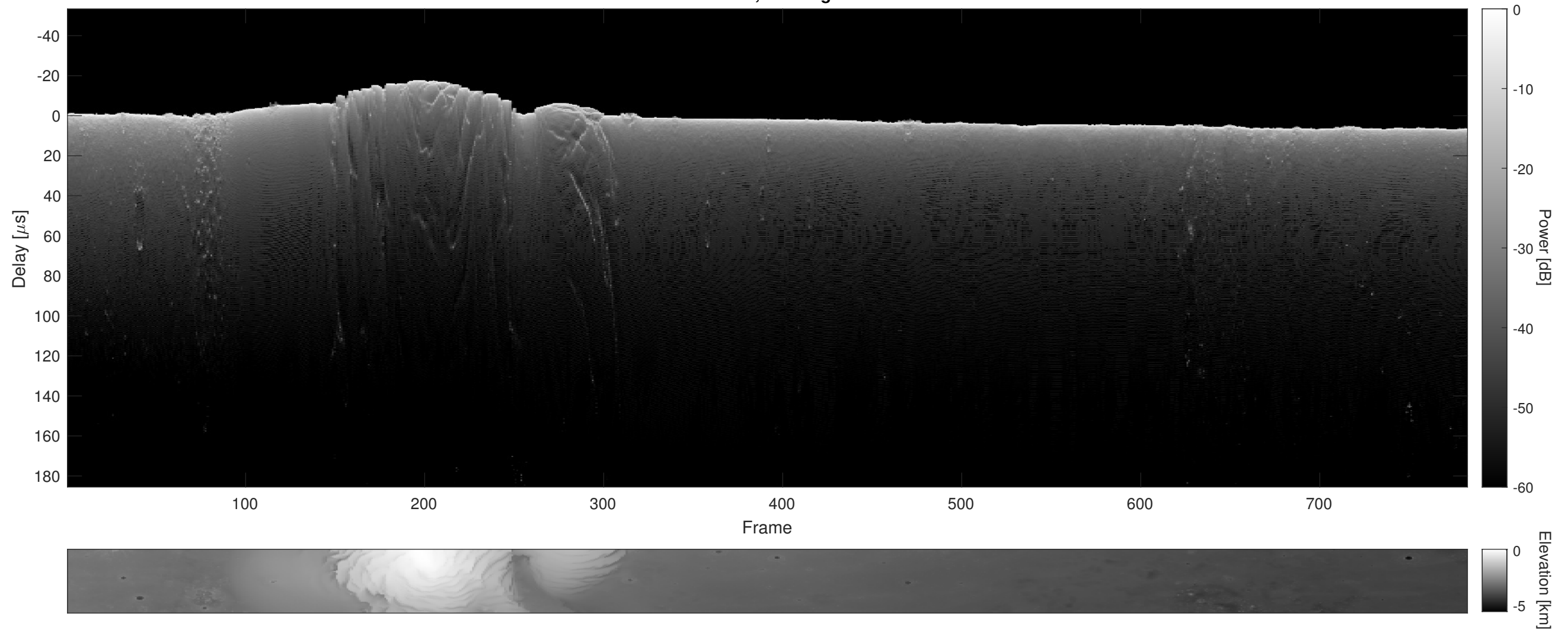
Orbit 9597, Cluttergram
