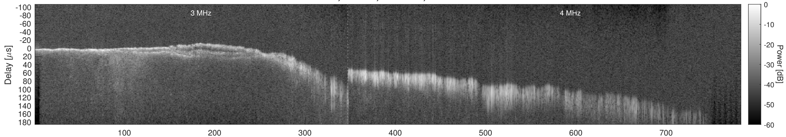
Orbit 9597, Window, Channel 2, Chapman
