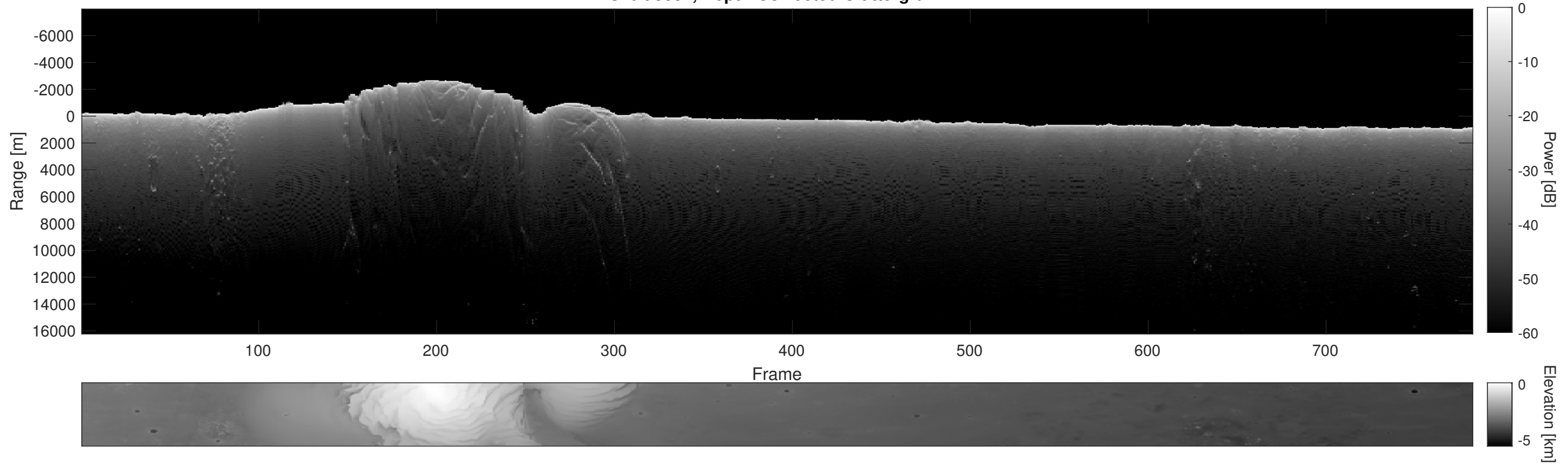
Orbit 9597, Depth-Corrected Cluttergram
