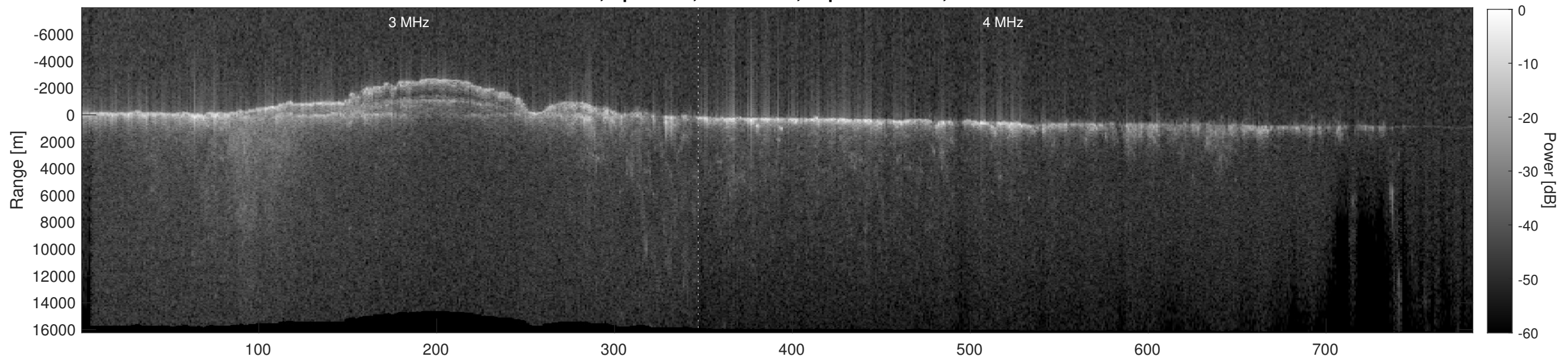
Orbit 9597, Depth-Corrected Cluttergram
