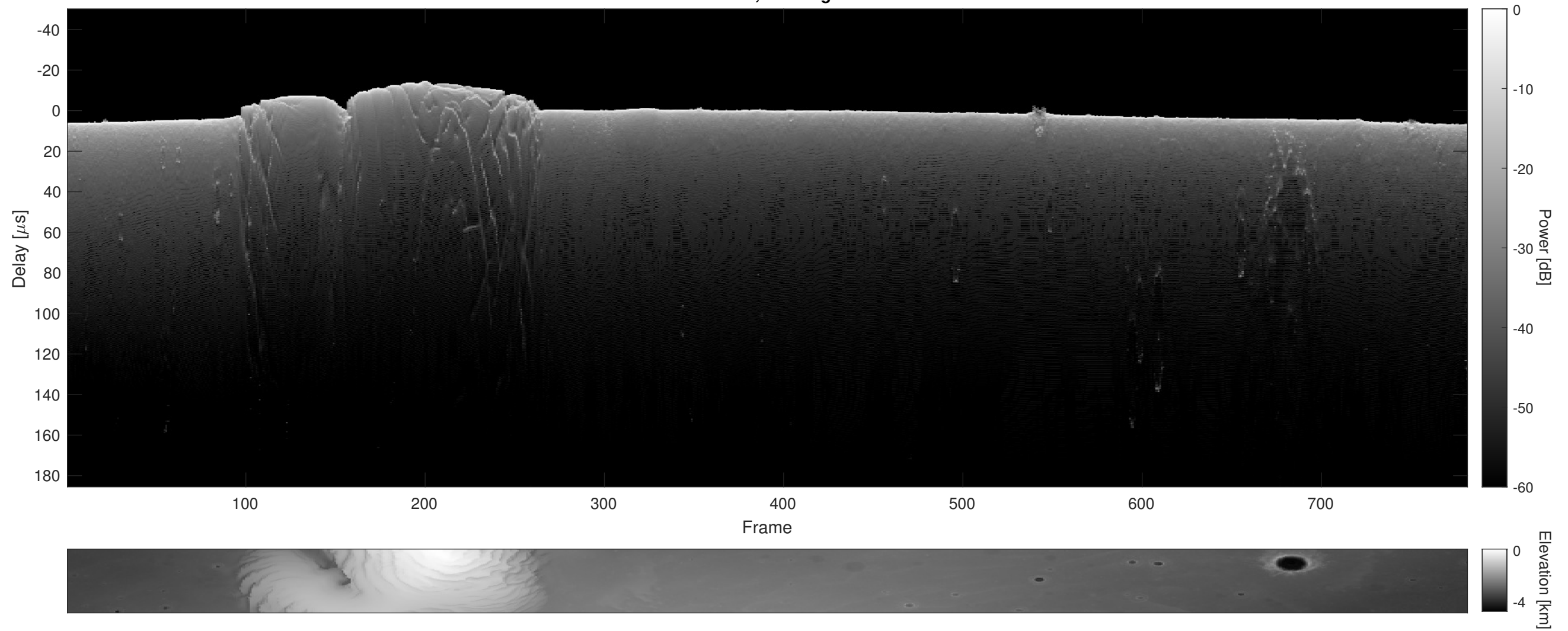
Orbit 9599, Cluttergram
