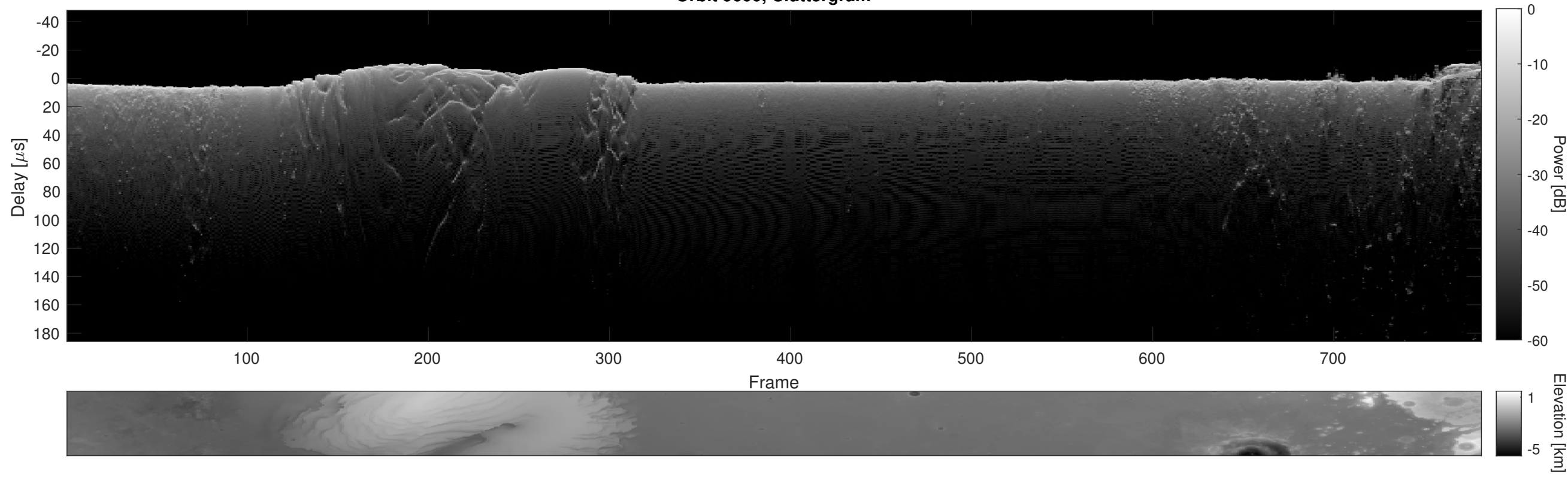
Orbit 9600, Cluttergram
