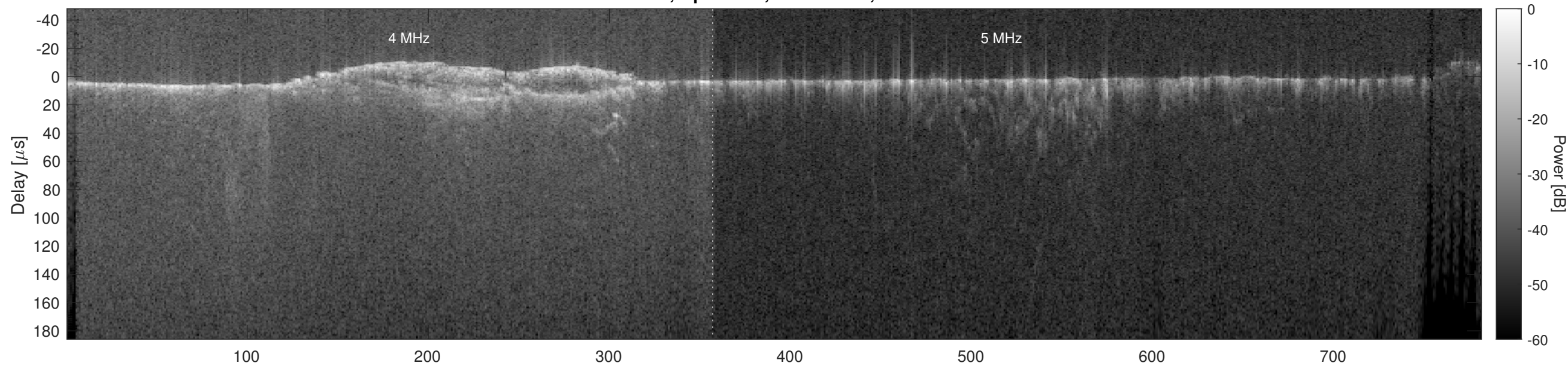
Orbit 9600, Optimized, No Window, Channel 2
