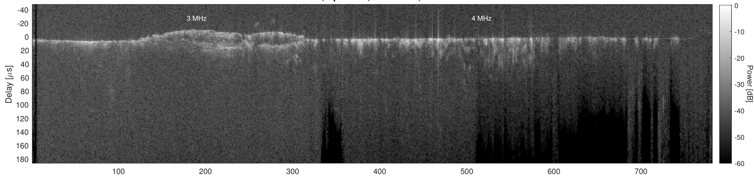
Orbit 9600, Cluttergram
