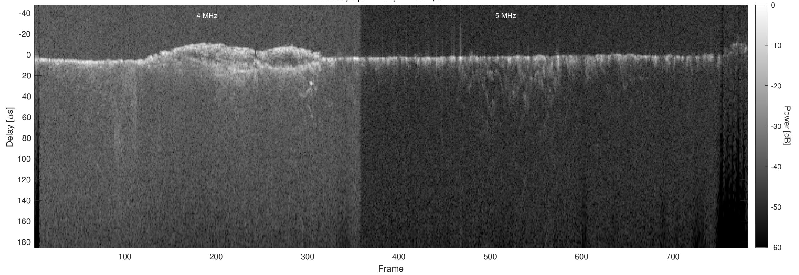
Orbit 9600, Optimized, Window, Channel 2
