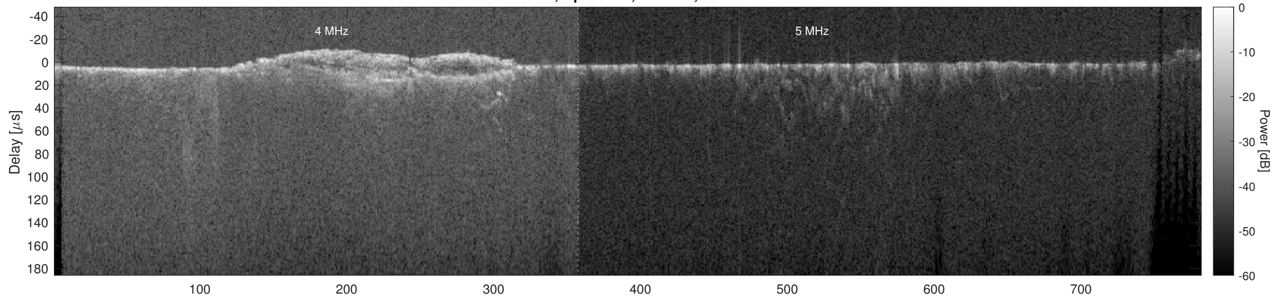
Orbit 9600, Optimized, Window, Channel 2
