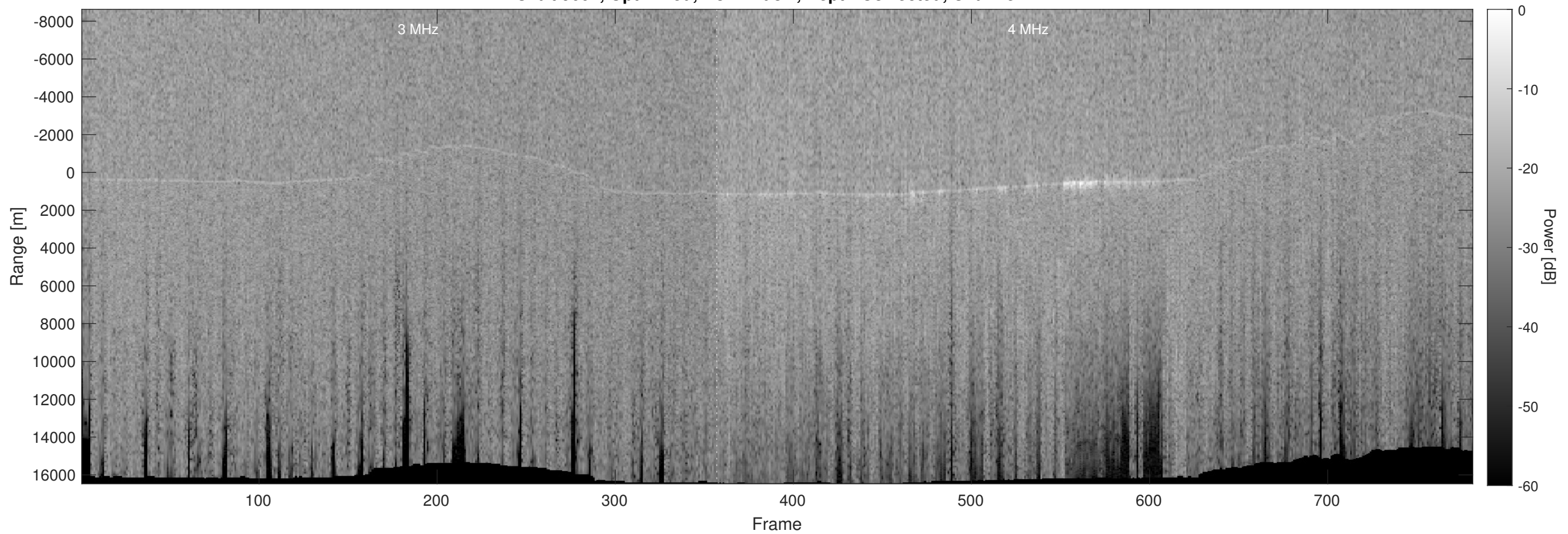
Orbit 9601, Optimized, No Window, Depth-Corrected, Channel 2
