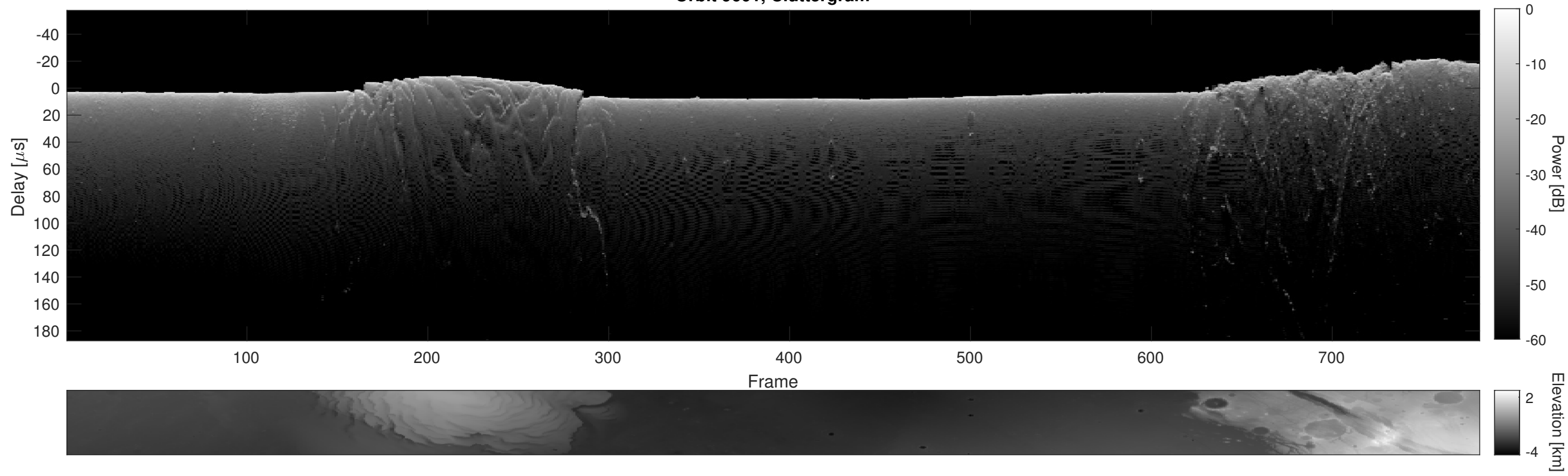
Orbit 9601, Cluttergram
