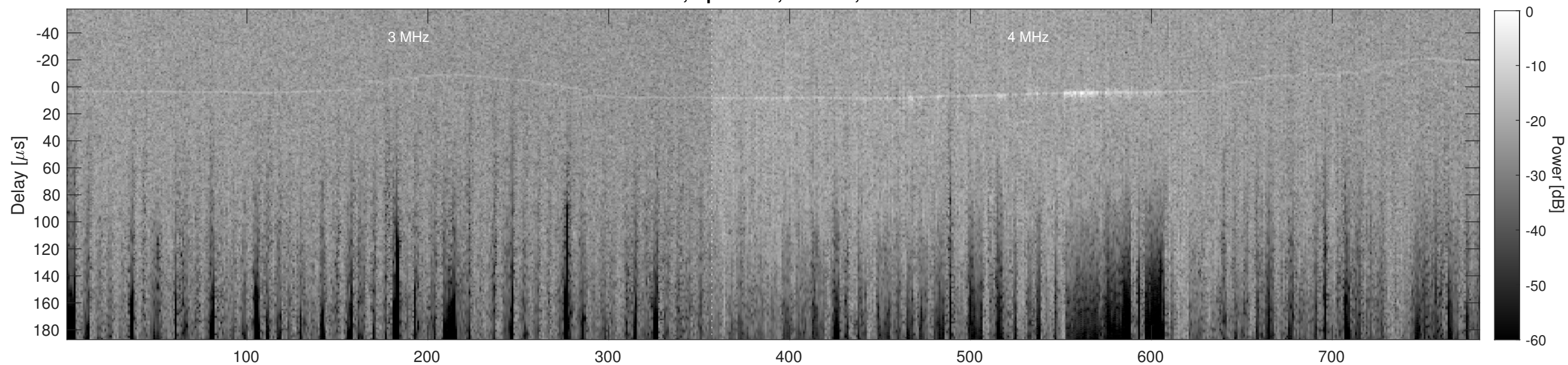
Orbit 9601, Cluttergram
