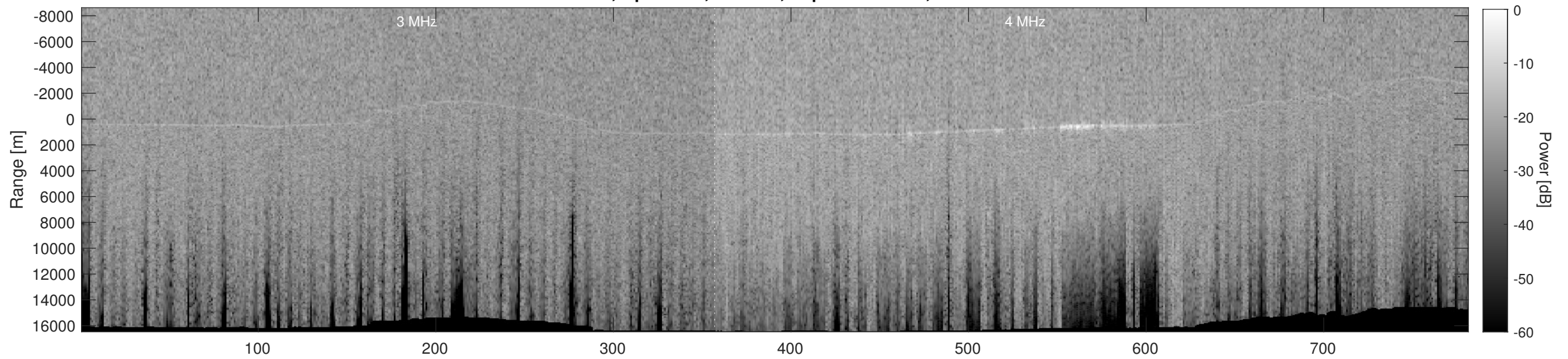
Orbit 9601, Depth-Corrected Cluttergram
