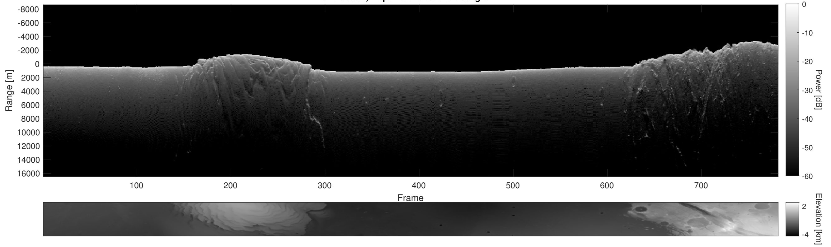
Orbit 9601, Depth-Corrected Cluttergram
