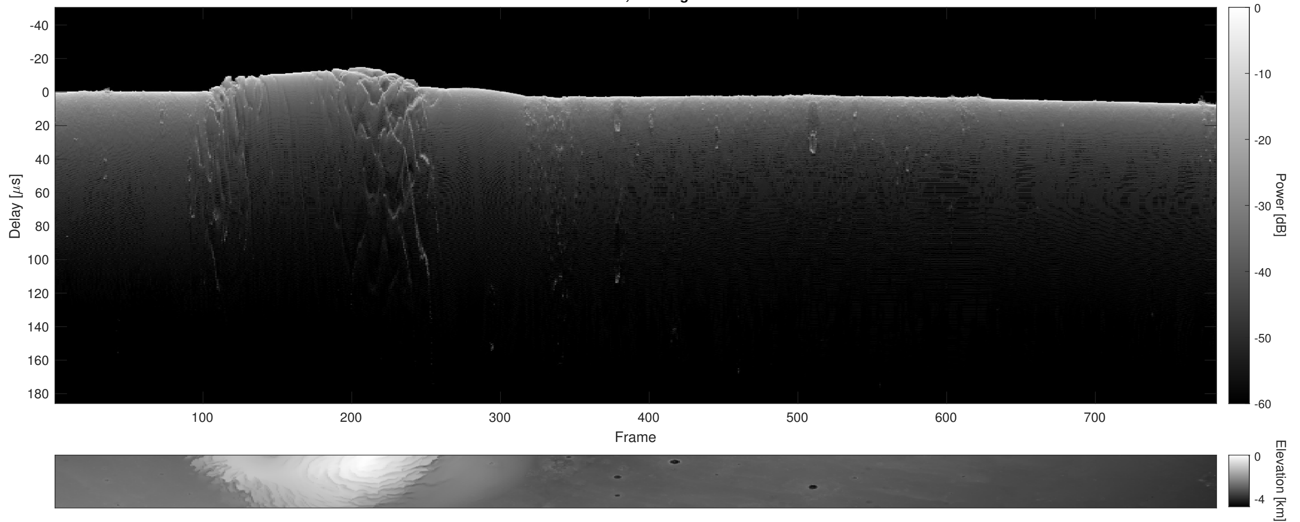
Orbit 9602, Cluttergram
