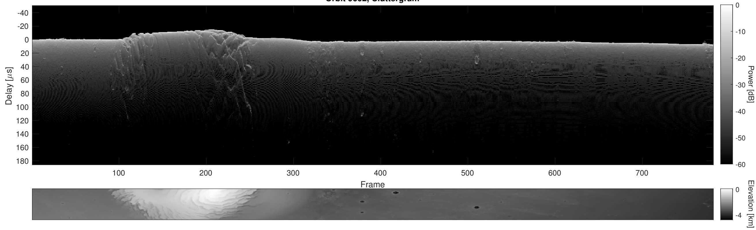
Orbit 9602, Cluttergram
