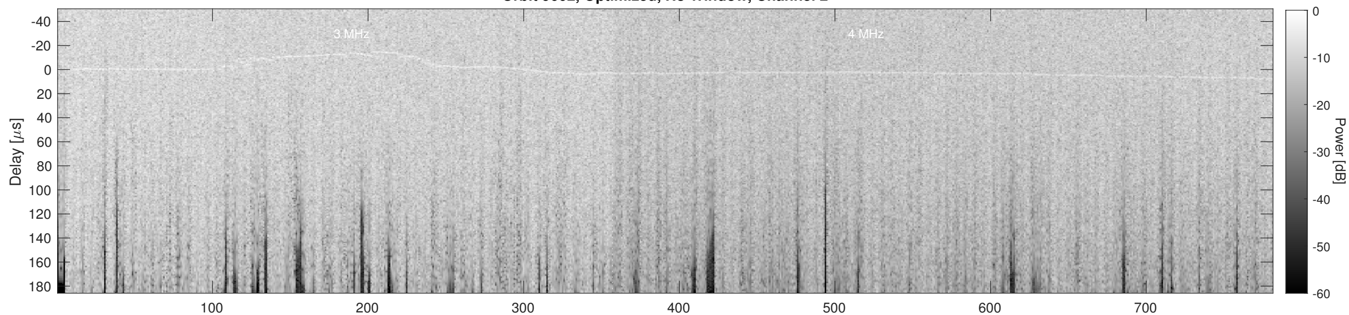
Orbit 9602, Cluttergram
