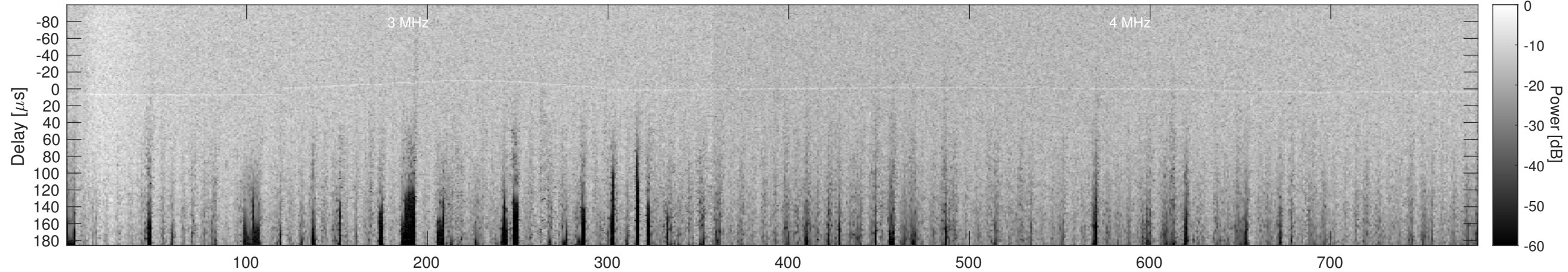
Orbit 9603, Cluttergram
