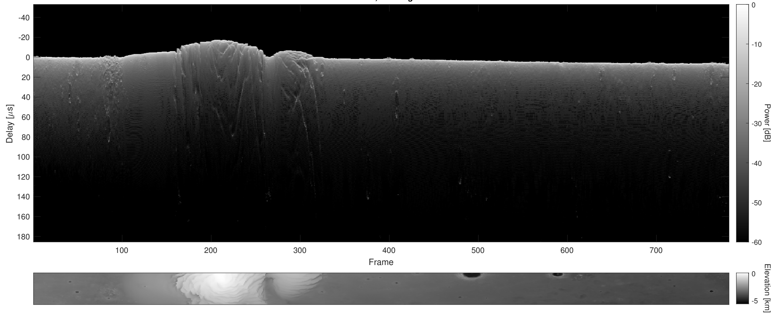
Orbit 9604, Cluttergram
