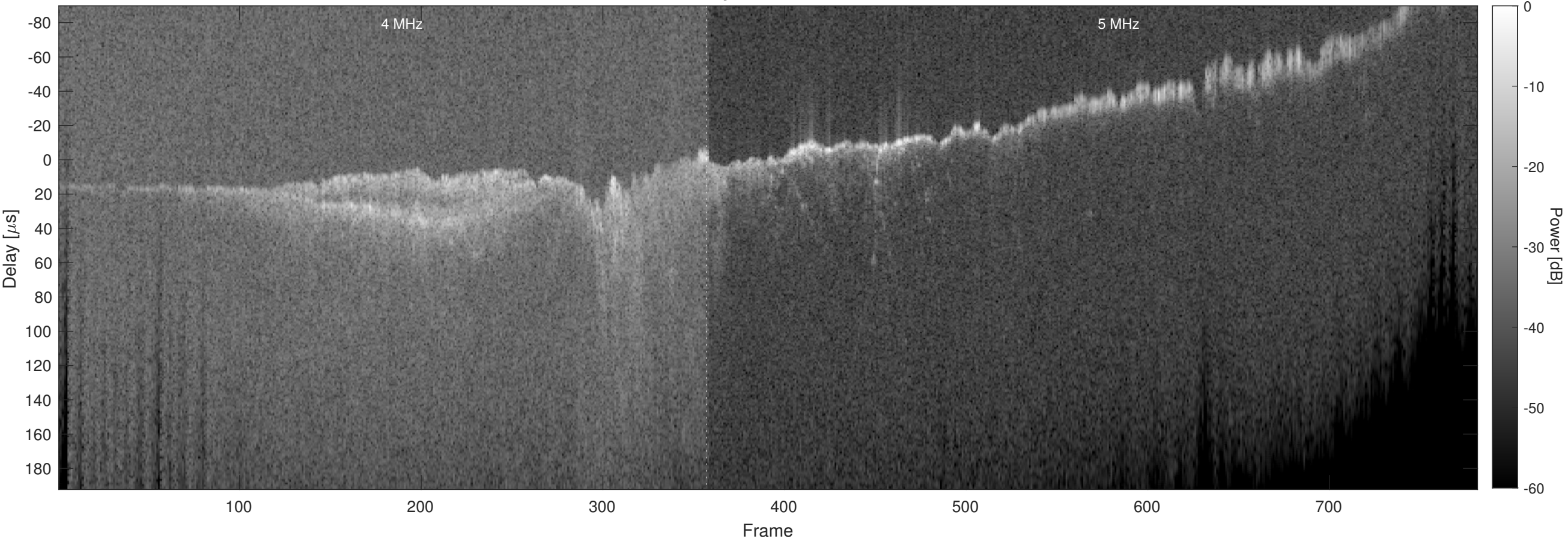
Orbit 9605, Chapman, Window, Channel 2
