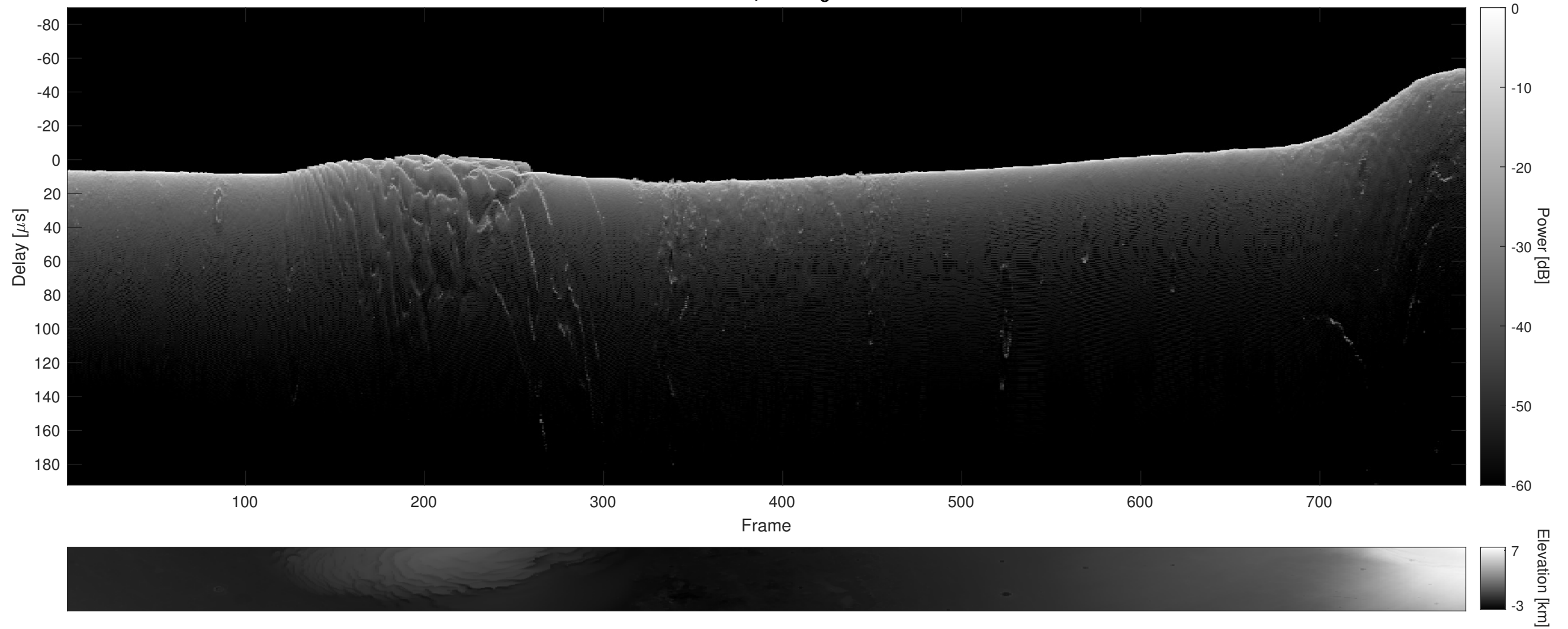
Orbit 9605, Cluttergram
