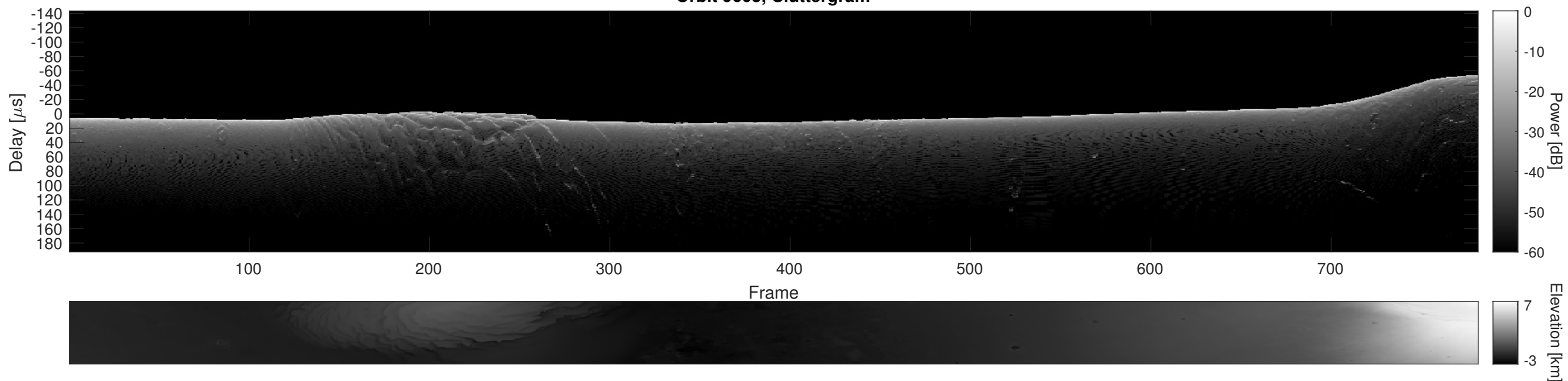
Orbit 9605, Cluttergram
