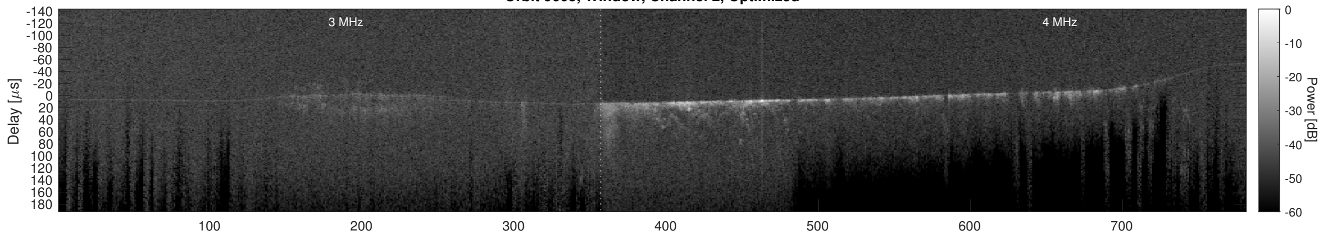
Orbit 9605, Cluttergram
