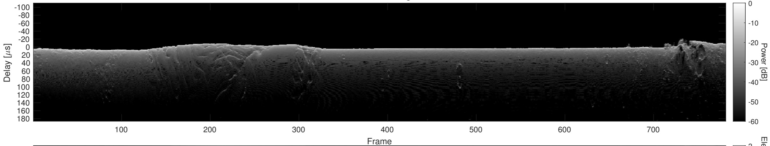
Orbit 9607, Cluttergram
