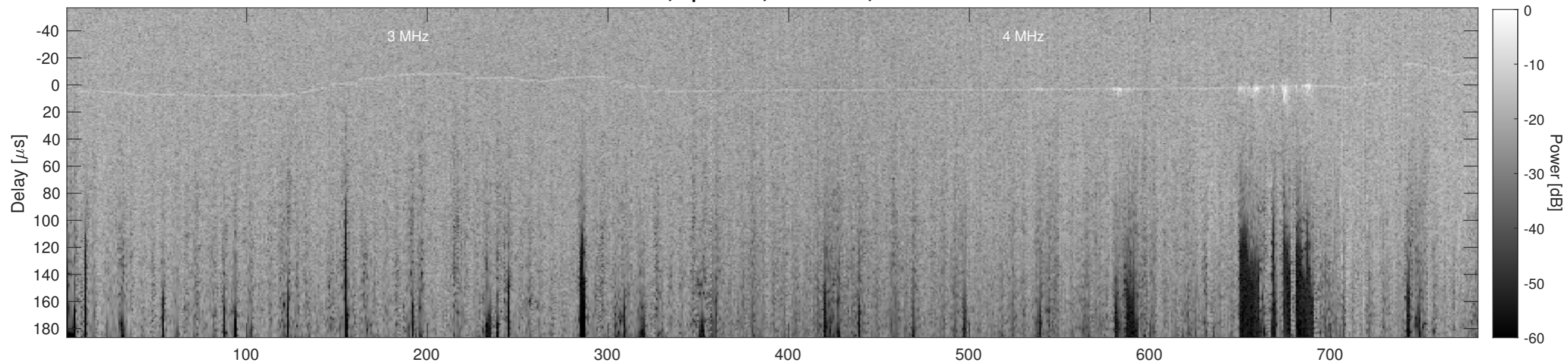
Orbit 9607, Cluttergram
