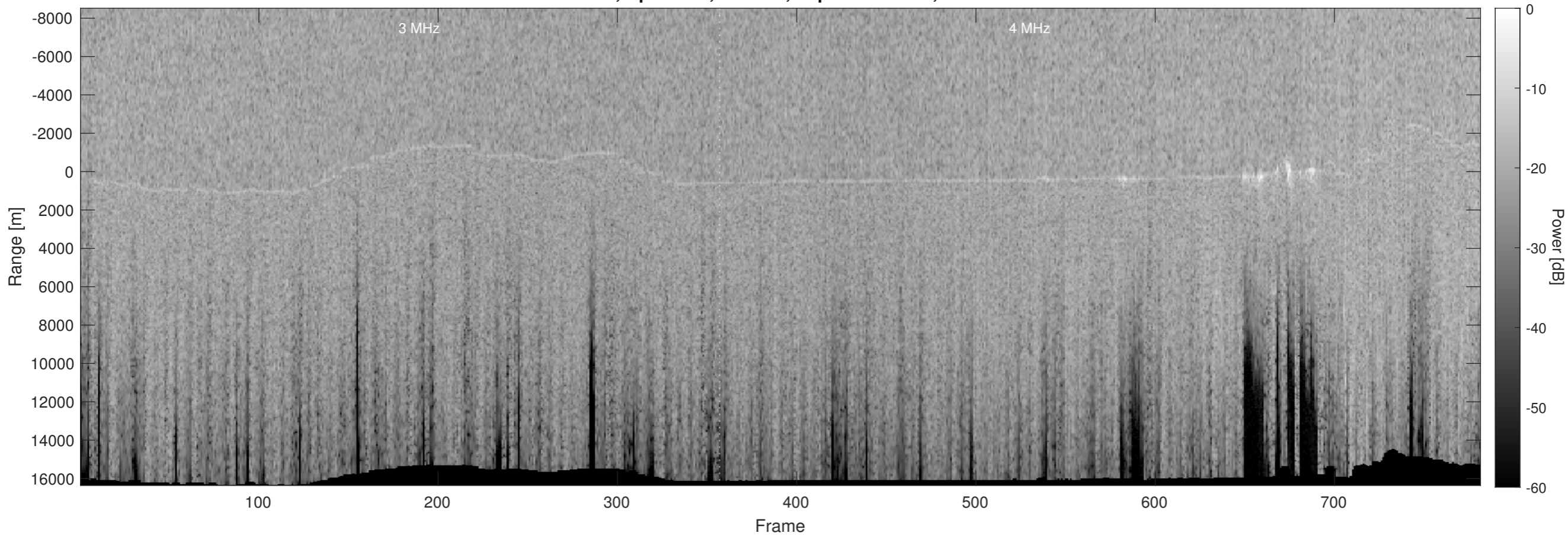
Orbit 9607, Optimized, Window, Depth-Corrected, Channel 2
