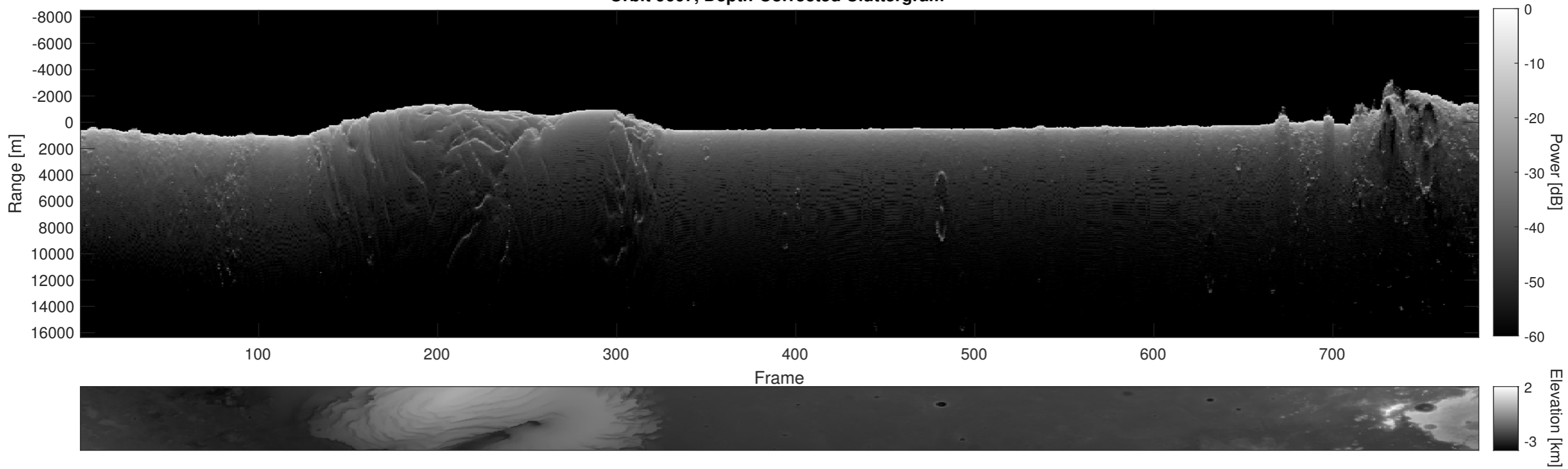
Orbit 9607, Depth-Corrected Cluttergram
