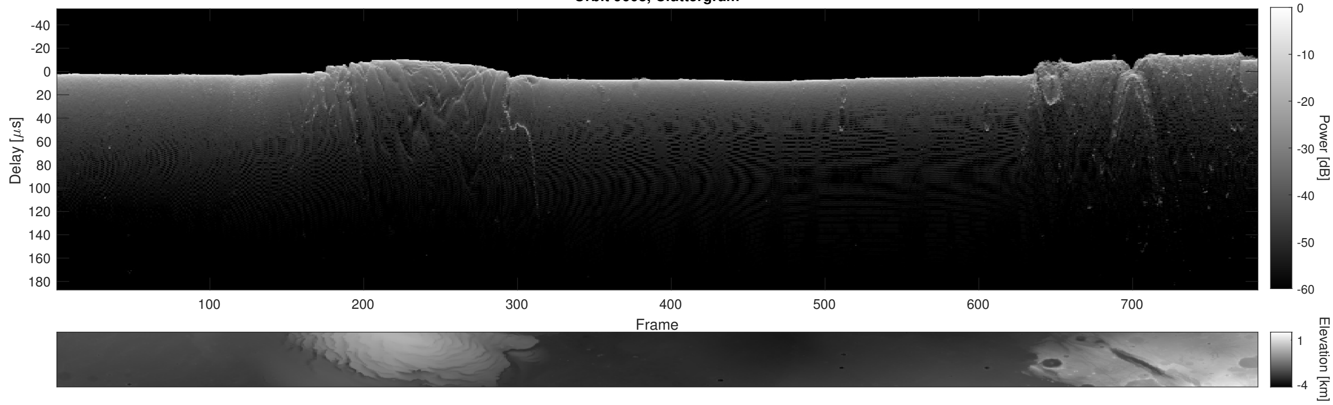
Orbit 9608, Cluttergram
