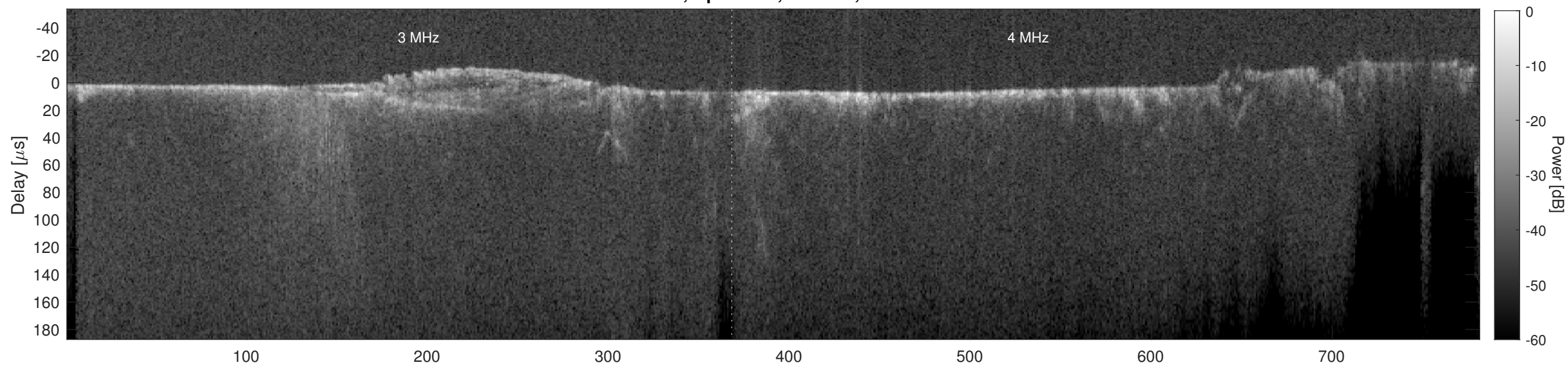
Orbit 9608, Cluttergram
