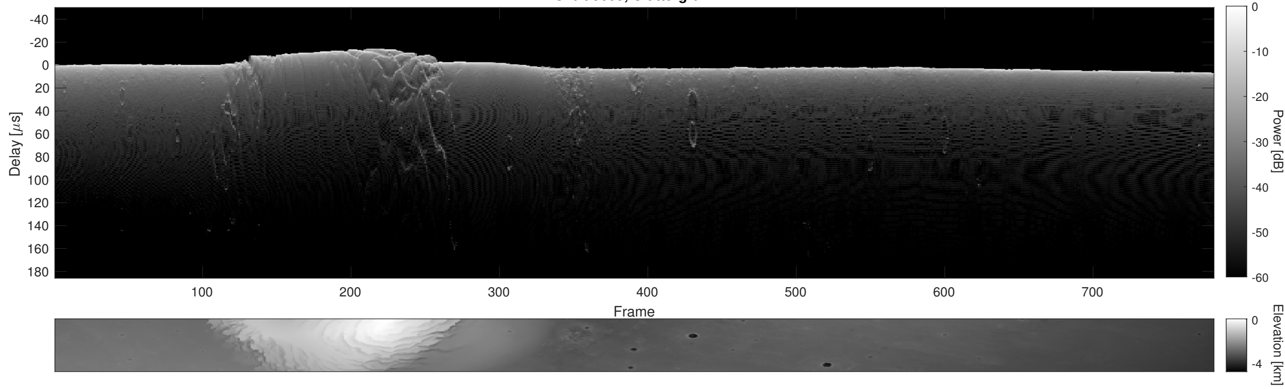
Orbit 9609, Cluttergram
