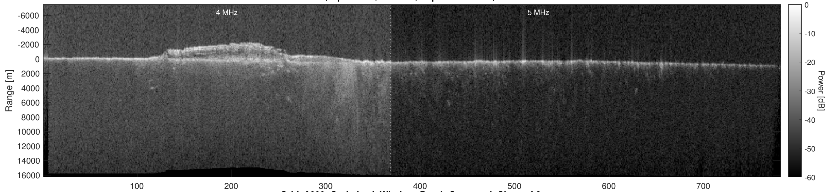
Orbit 9609, Optimized, Window, Depth-Corrected, Channel 2
