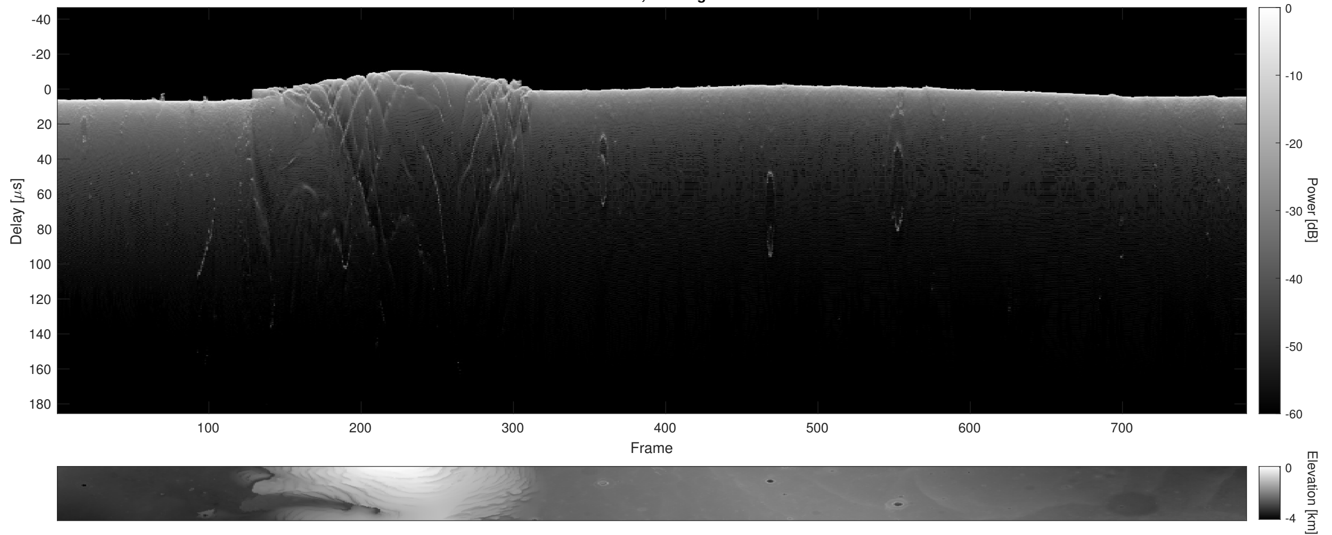
Orbit 9610, Cluttergram
